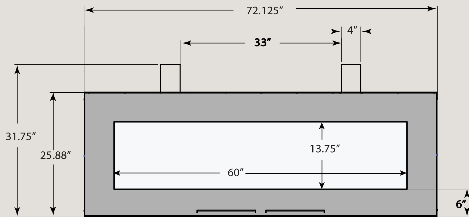
Front view
