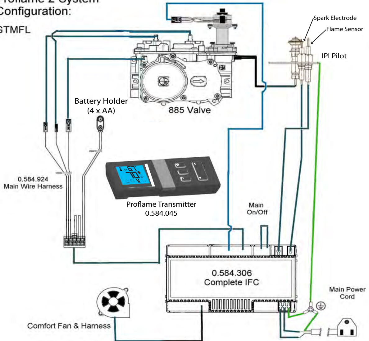
Figure 55: Wiring diagram.
