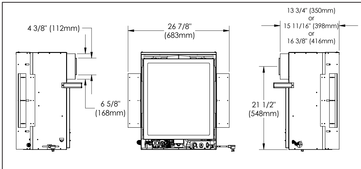
Figure 2. Q1CI Dimensions - Rear Vent
