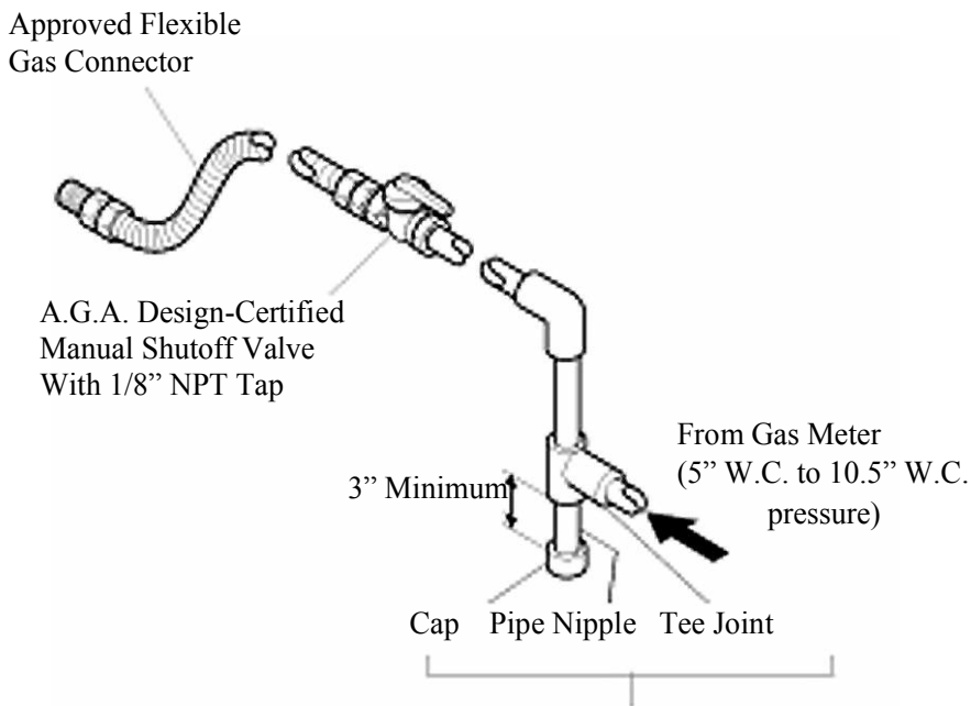
Figure 1 - Sediment Trap
