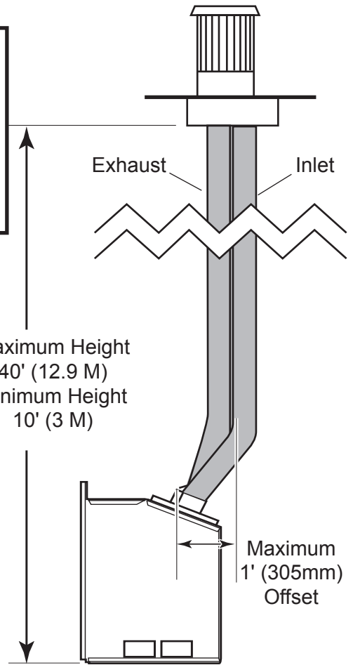
Figure 5 - Venting Unit
