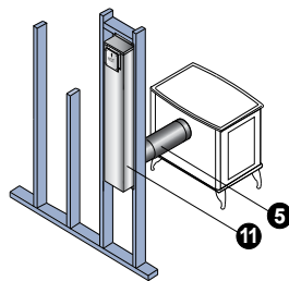
Stove with Snorkel Horizontal Termination
