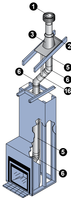
Fireplace Vertical Termination
