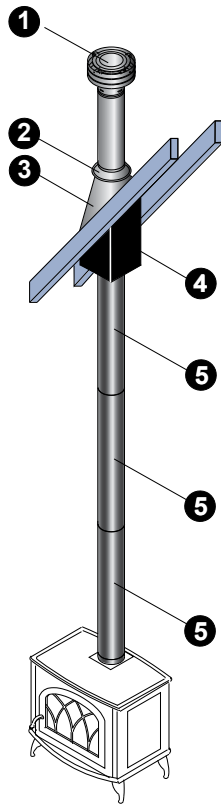
Cathedral Ceiling Stove Installation
