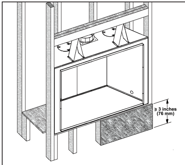
Figure 17. Raised Fireplace with no Hearth
