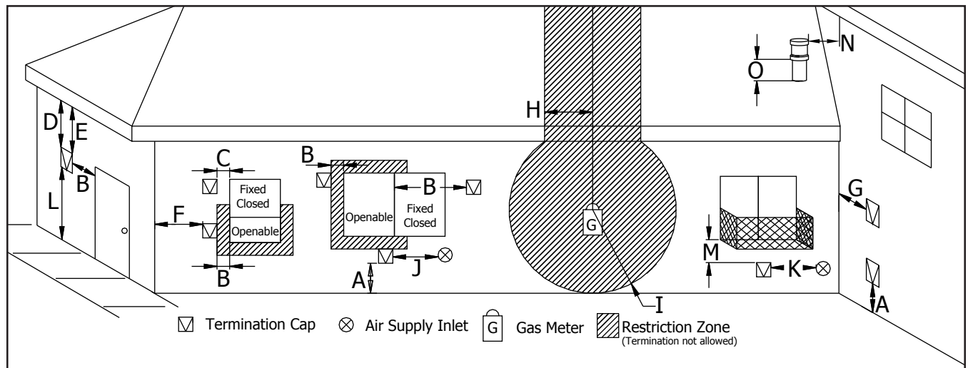
Figure 24. Vent Termination Restrictions, refer to Table 2.
