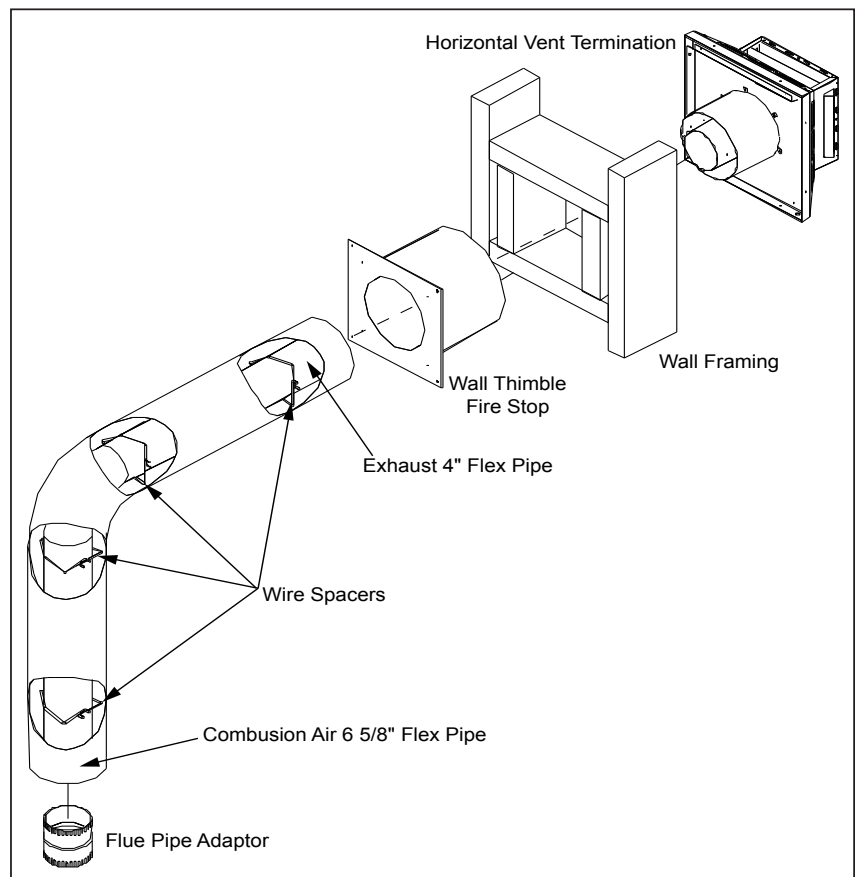
Figure 27: Installation of Fireplace Horizontal Vent Kit.
