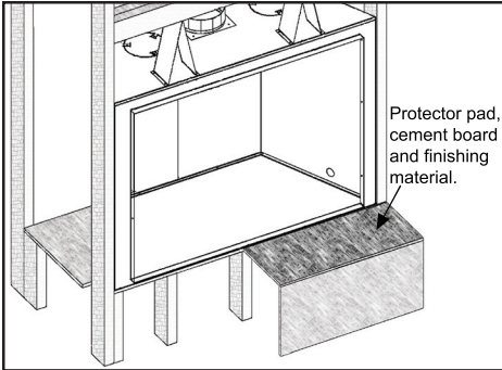
Figure 19. Raised Fireplace with Raised Hearth
