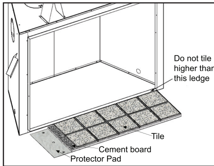
Figure 20. Floor Level Hearth Requirements
