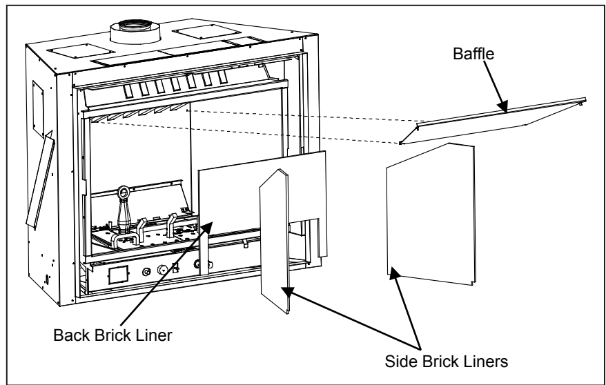
Figure 43: Cast Iron Brick Liner Installation.
