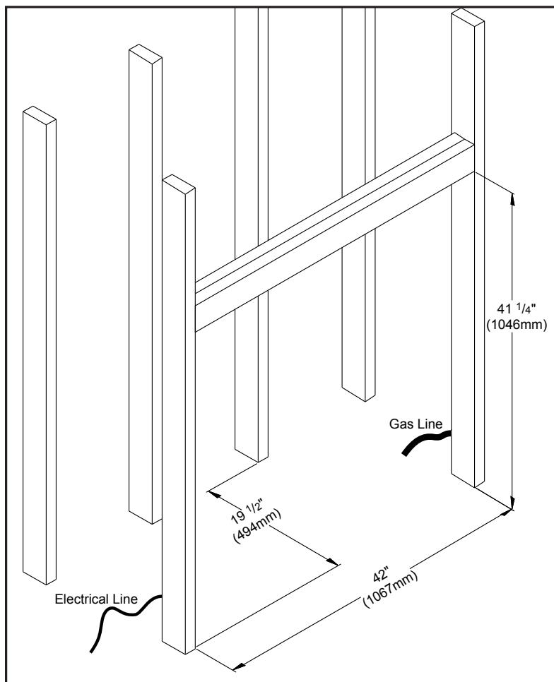
Figure 15. Dimensions for Framing the Firebox.
