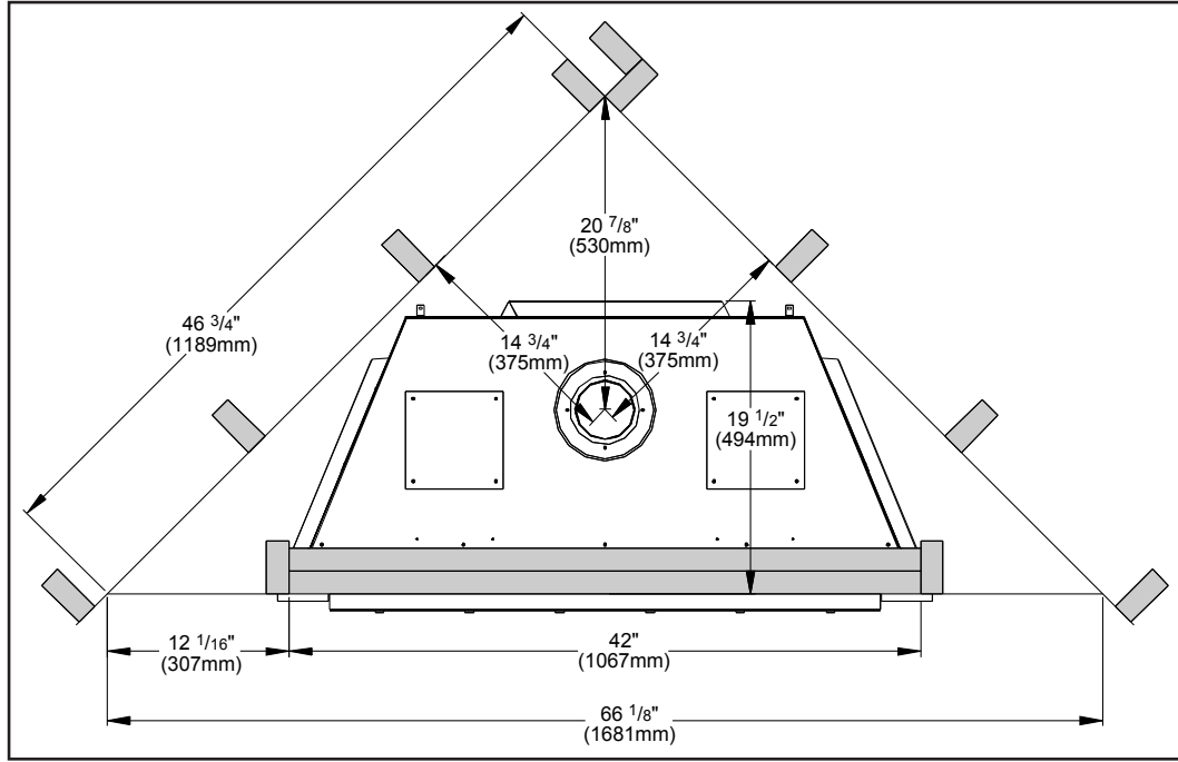
Figure 16. Dimensions for a corner installation.
