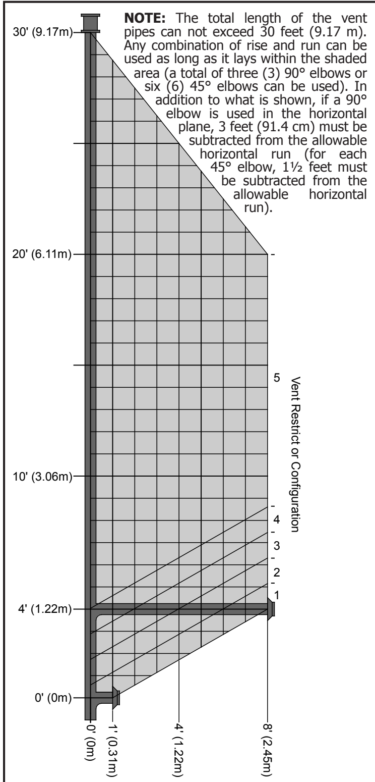
Figure 30. Possible Vent Configurations
