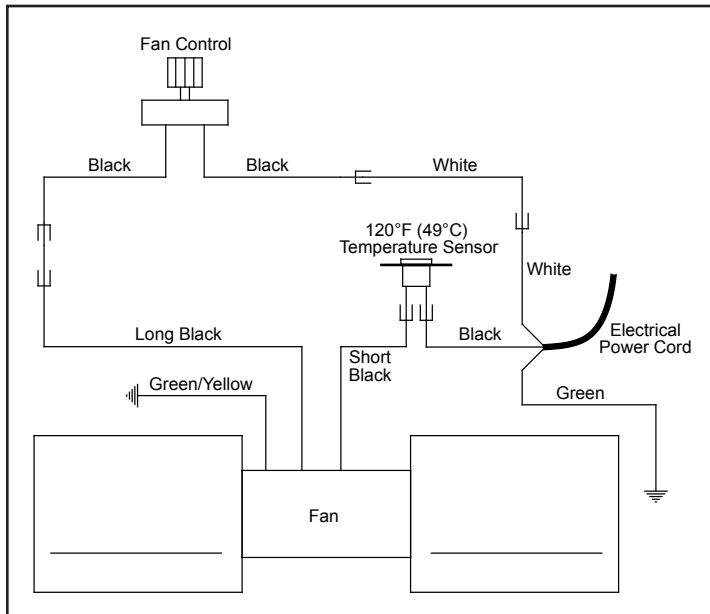
Figure 40. Wiring Diagram For Fan Control.
