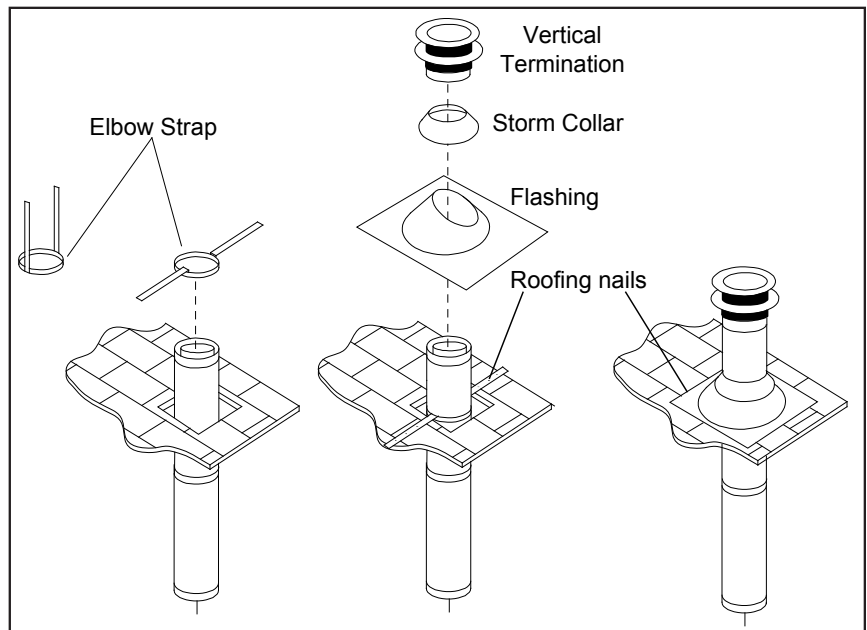
Figure 33. Vertical Vent Termination
