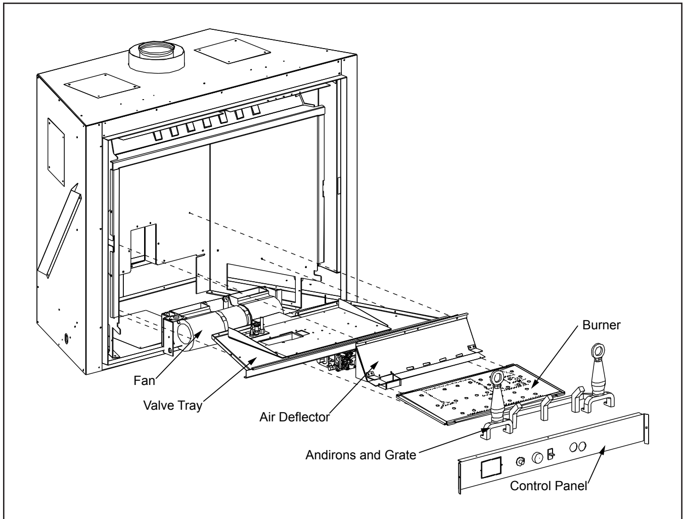
Figure 9: Removal of DV42DX Burner and Fan.
