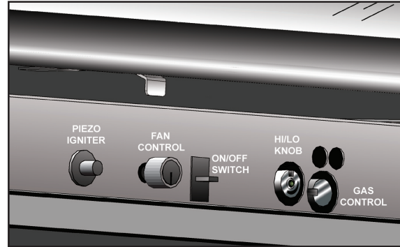
Figure 6. Control Panel
