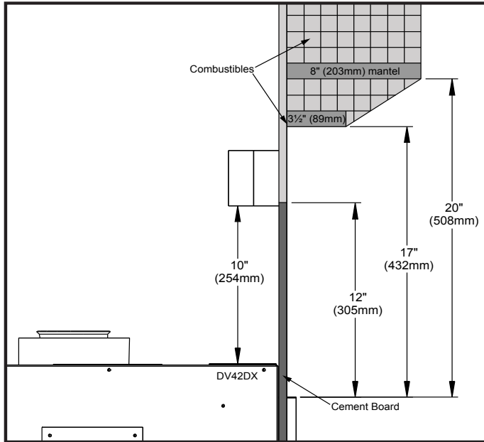
Figure 22. Combustible Mantel Clearances.
