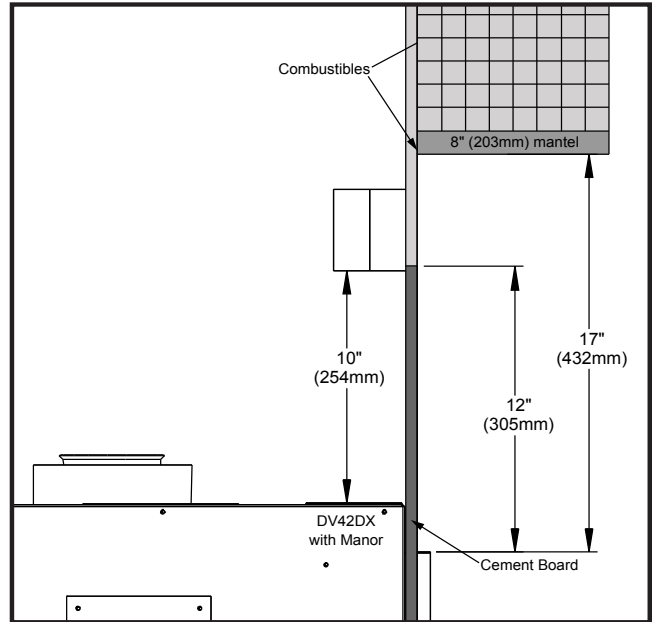
Figure 23. Combustible Mantel Clearances for The Manor
