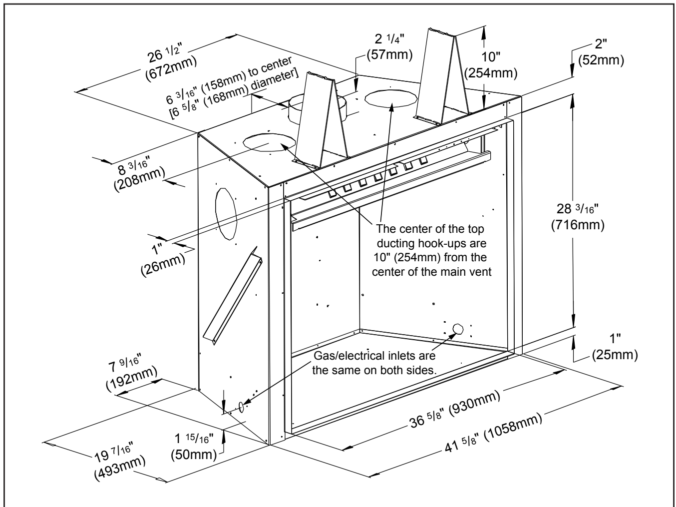
Figure 1. Dimensions of the Firebox.
