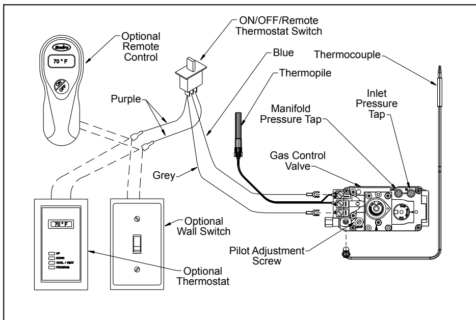
Figure 41. Wiring Diagram For Gas Valve.
