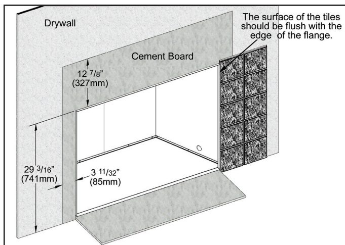
Figure 21. Dimensions Facing Around Opening.
