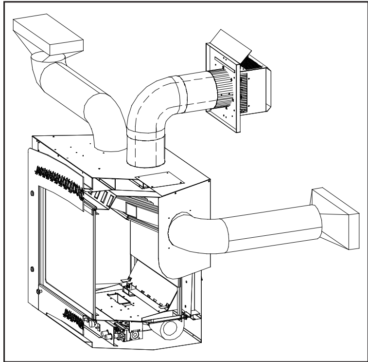
Figure 37. Heat Dumping Options.
