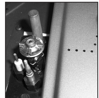
Figure 14. Ignitor assembly beside the burner.
