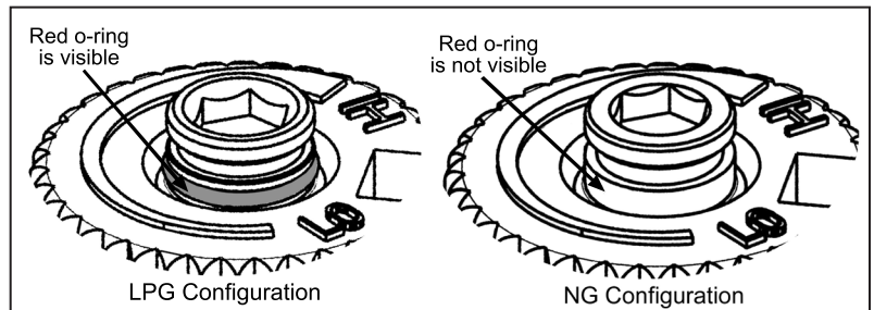
Figure 13: O-ring on valve screw.
