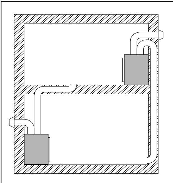
Figure 38. Ducting Options; ducted from upper floor to lower floor & from lower floor to upper floor.
