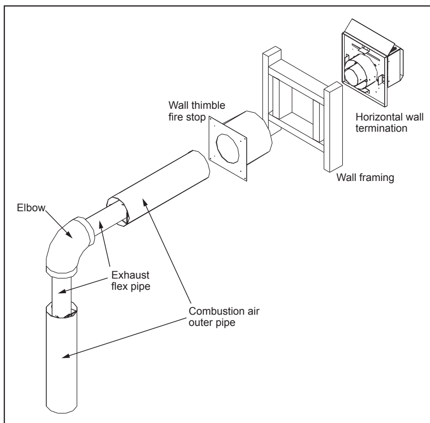
Figure 32. Horizontal Vent Termination
