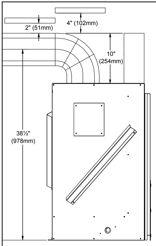
Figure 28. Hard Vent Pipe Clearances.
