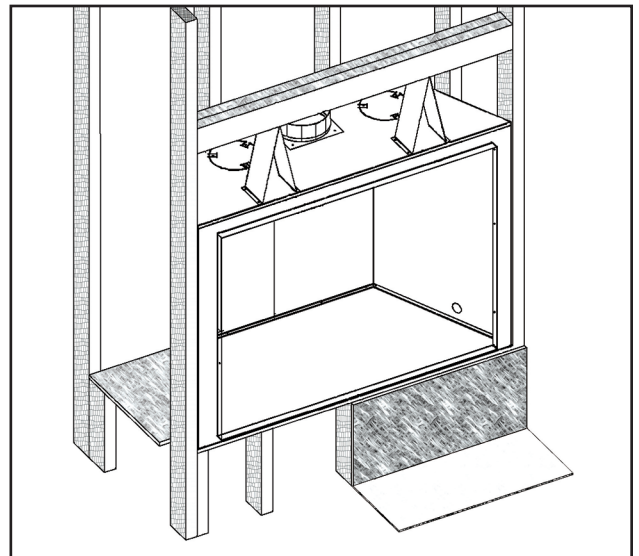
Figure 18. Raised Fireplace with Floor Level Hearth
