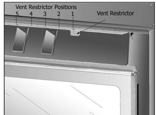
Figure 31. Possible Vent Configurations
