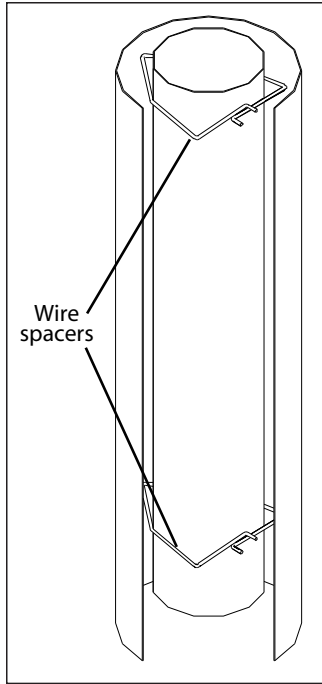
Figure 25: Wire Spacers.
