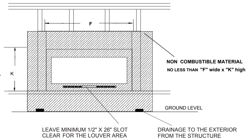
Figure 1.1 - Installation of facing materials ( Case #1)
