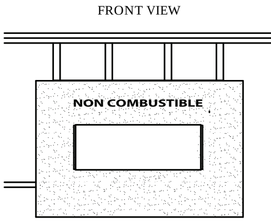
Figure 1.3 - Installation of facing materials ( Case #3)
