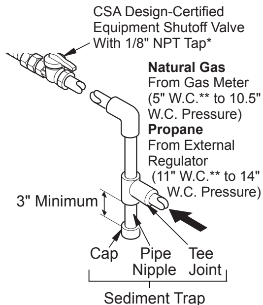
Figure 4 - Gas Connection
