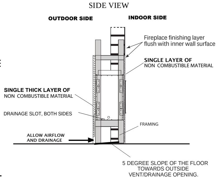
Figure 1.3 - Installation of facing materials ( Case #3)
